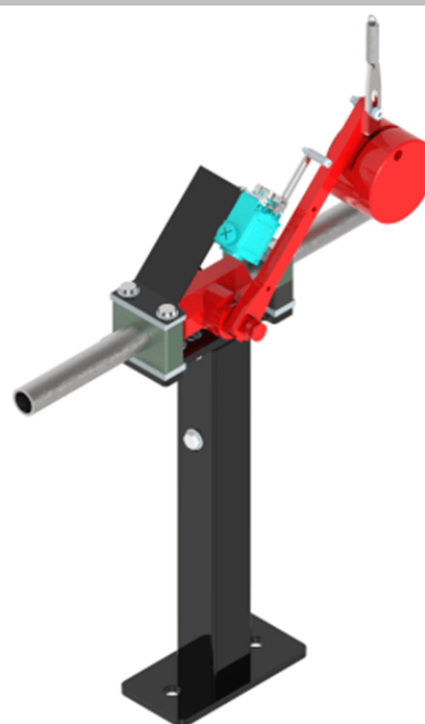
Image showing Free Fall Fire Valve arrangement fitted on bracket weight, link and tension spring with switch and bracket.
